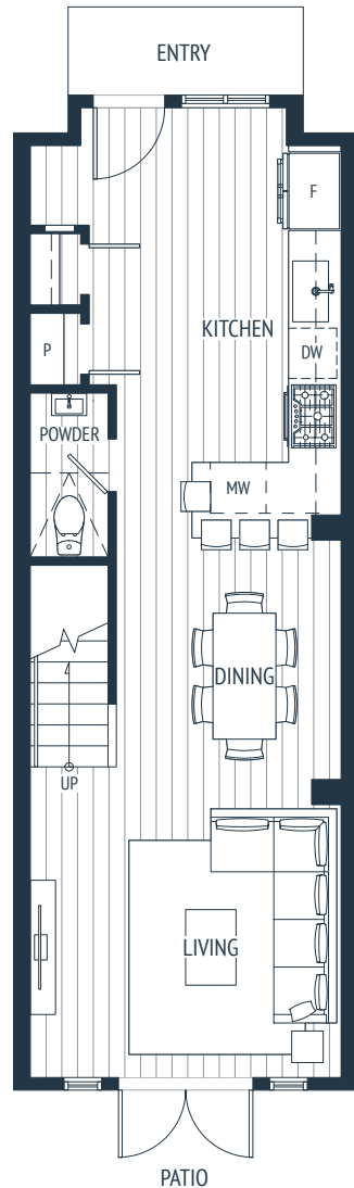
LOWER LEVEL
